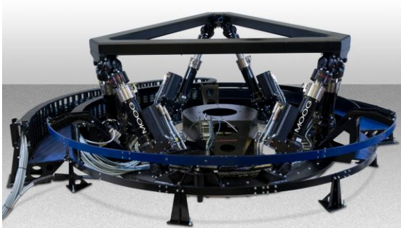
Motion system on turntable
