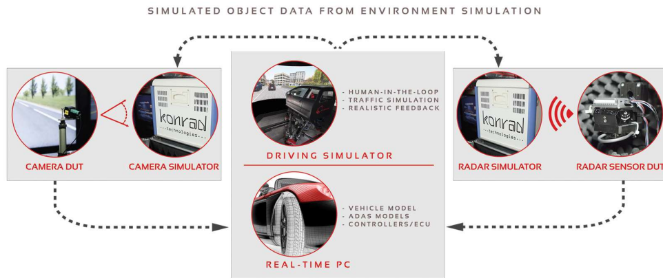
Figure 1: DIL with Sensor Fusion Test Top Level Architecture
